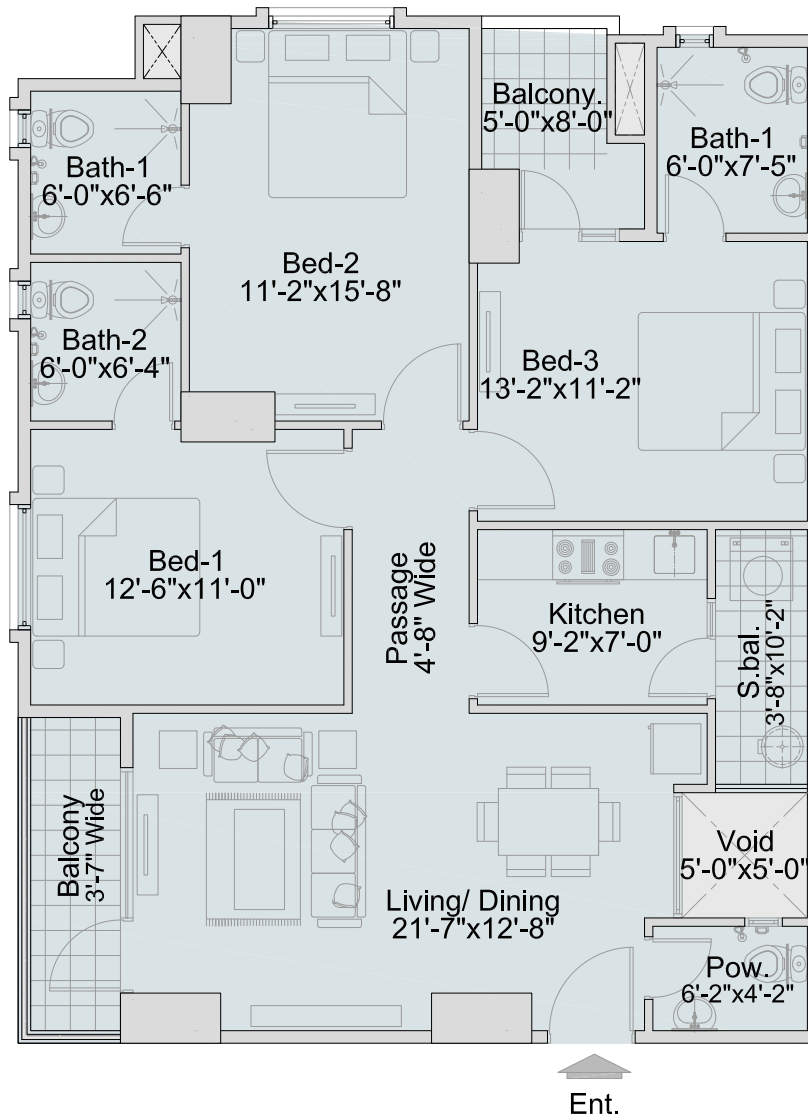
TYPE B1 - 3 BED
