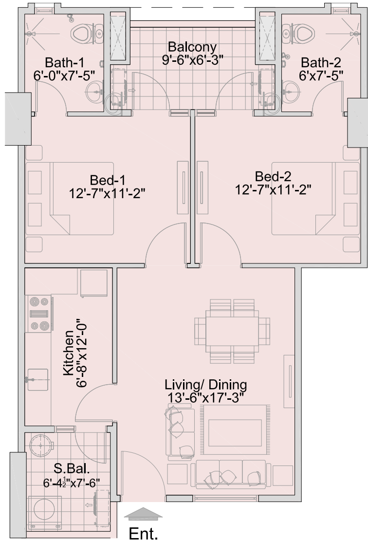
TYPE C3 - 2 BED
